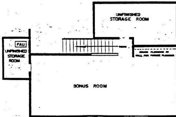
SECOND FLOOR STANDARD BONUS ROOM
